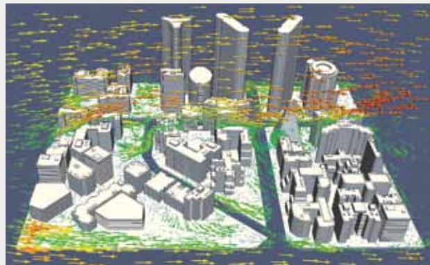
IHPC's researchers utilised their computational science expertise and the principles of fluid dynamics to accurately model, simulate and visualise wind flow patterns in a city.
