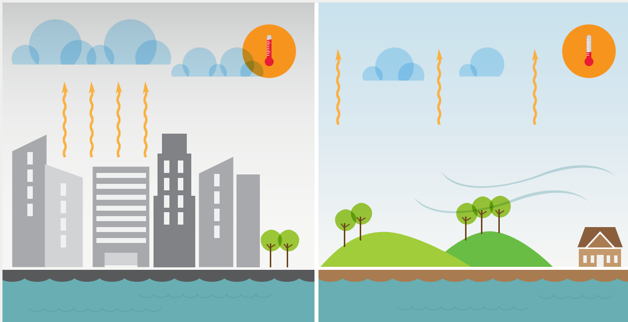
An urban heat island is a metropolitan area which is significantly warmer than its surrounding rural areas. The temperature difference is usually higher at night than during the day, and is most apparent when winds are weak.
