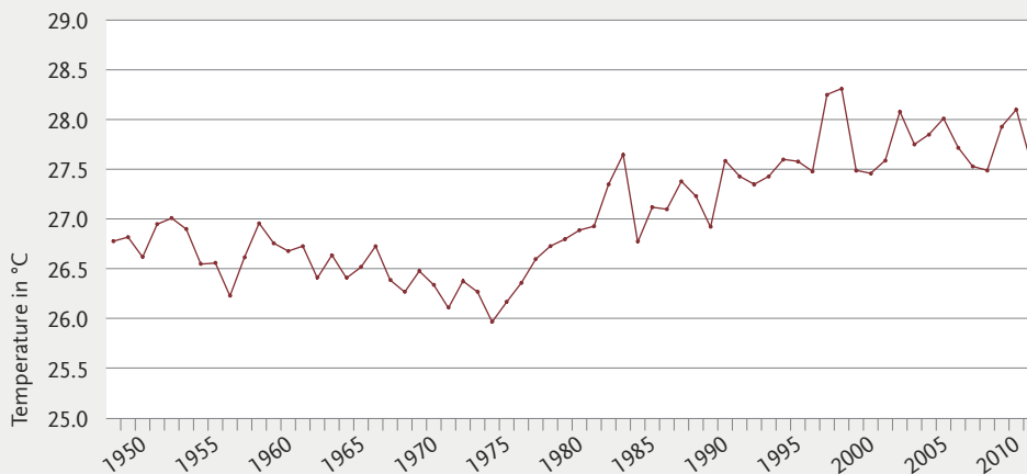
Figure 4.2: Annual Mean Surface Temperature (°C)
